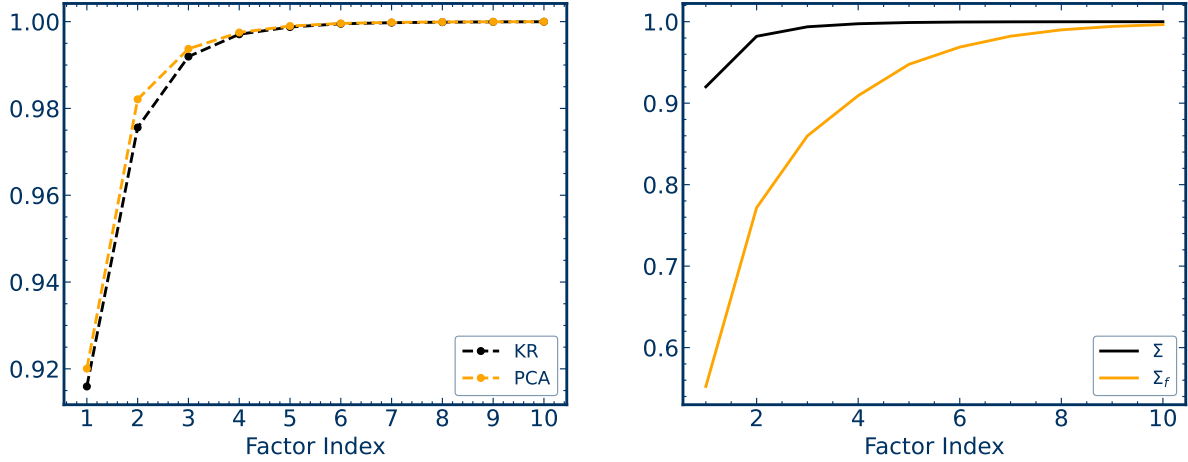
(a) Explained variation in discount bond excess returns for KR and PCA factors (b) Normalized cumulative sum of eigenvalues of \Sigma and \Sigma_f
